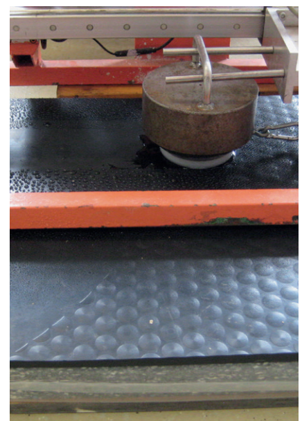
Figure 5: Slip resistant measurement
