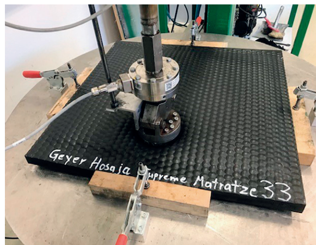
Figure 4: Permanent tread load test
