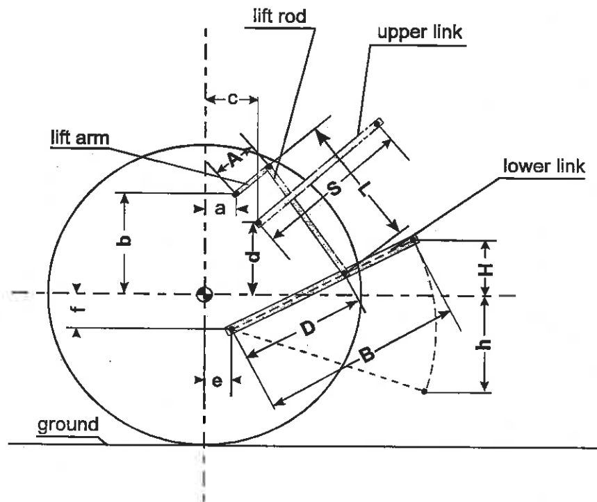
Figure 2.1 Lift Test – Linkage geometry
