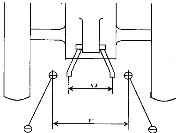
Figure 2.2 Lift Test – Linkage geometry
