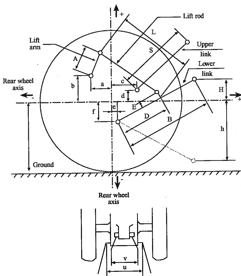
LIFT TEST Linkage geometry
