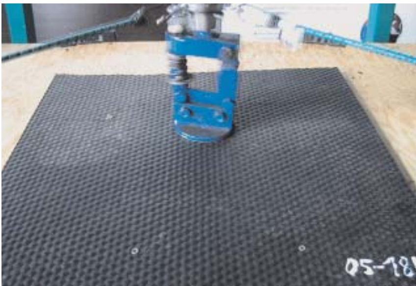
Bild 2: Continuous tread load test with an artificial cow's foot
